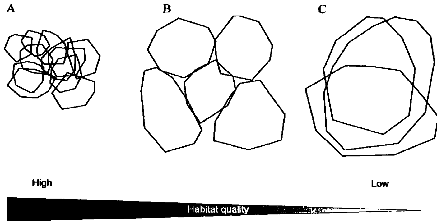
Fig. 6.1. The spatial organization of individuals varies along a continuum according to habitat quality, which can be defined by the abundance and predictability of food resources. A. In areas of high quality habitat, populations are characterized by high densities, small home ranges, and high home range overlap. B. In areas of intermediate quality habitat, populations are characterized by intermediate densities, moderately-sized home ranges, and low levels of home range overlap. C. In areas of low quality habitat, populations are characterized by low densities, large home ranges, and high home range overlap.
