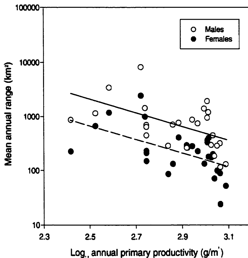
Fig. 4.4. Mean annual ranges (km 2 ) of grizzly bears for selected North American populations versus log 10 mean annual primary productivity (g/m 2 ). The equation for the male regression line (solid line) is y = 1620000 - 17.4x . The equation for the female regression line (dashed line) is y = 1170000 - 17.4x . R^2 for the ANCOVA was 0.45. Presented in McLoughlin et al. (1999) and reprinted with permission from the International Bear Association.
