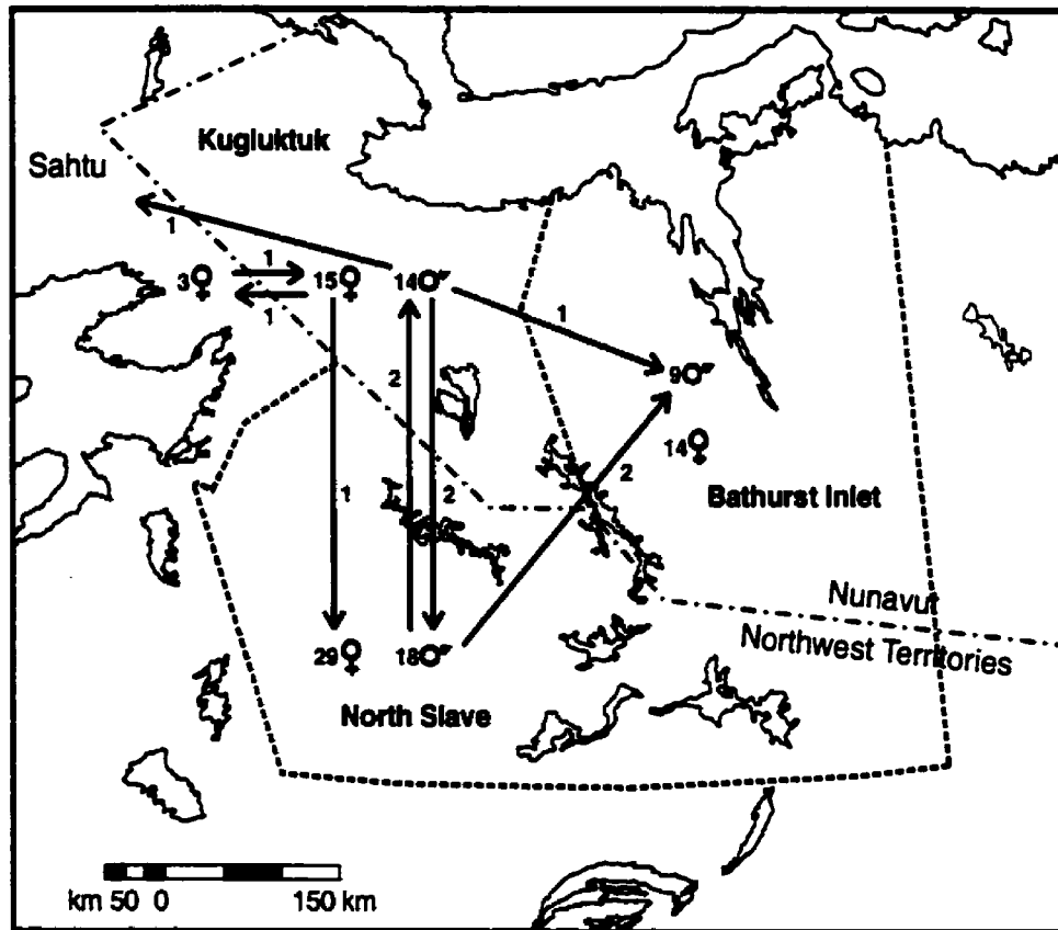
Fig. 2.8. Final boundaries of grizzly bear populations for the North Slave, Bathurst Inlet, and Kugluktuk clusters in the central Arctic. Boundaries were based on the 70% utilization distributions (fixed kernel) for male and female populations. Immigration and emigration after one bear-year of data (see text) are indicated for the female and male components of each population unit. Arrows indicate direction of exchange and number and sex of animals immigrating or emigrating across population boundaries. Numbers next to gender symbols indicate the number of resident bears of a sex originating in a population unit.
